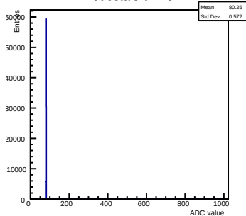
Pedestals ch 13
