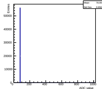
Pedestals ch 10
