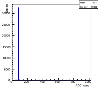
Pedestals ch 1
