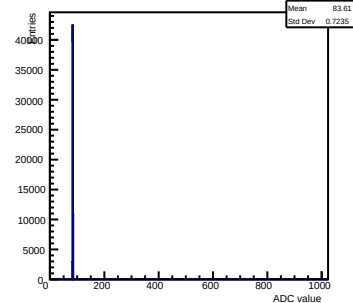
Pedestals ch 4
