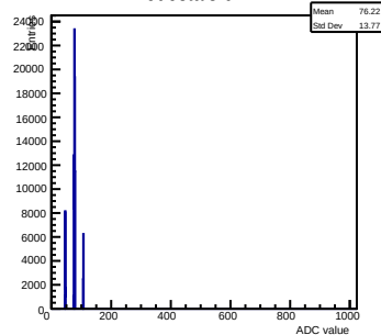
Pedestals ch 14
