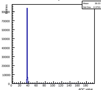
Pedestals ch 13 chip 65 incm=0.9
