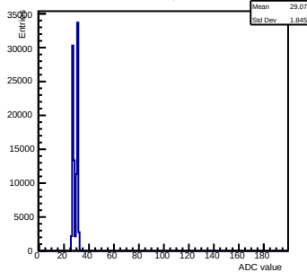
Pedestals ch 2 chip 65 incm=1.0
