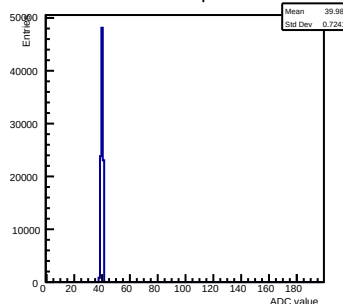
Pedestals ch 15 chip 65 incm=0.9
