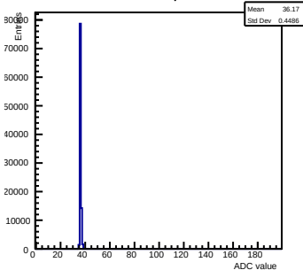
Pedestals ch 13 chip 65 incm=1.0
