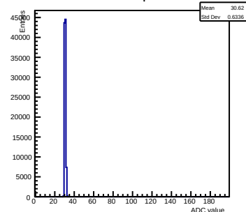
Pedestals ch 12 chip 65 incm=0.9
