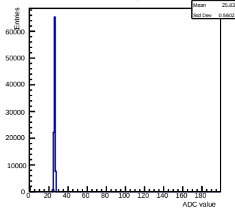
Pedestals ch 10 chip 65 incm=1.0
