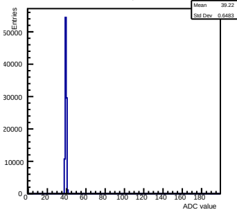
Pedestals ch 1 chip 65 incm=0.8
