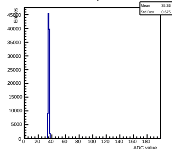
Pedestals ch 4 chip 65 incm=0.9
