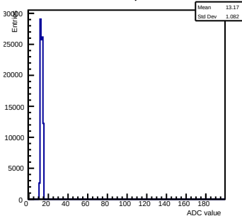
Pedestals ch 5 chip 65 incm=1.0
