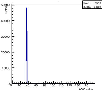
Pedestals ch 13 chip 65 incm=0.8
