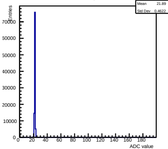
Pedestals ch 9 chip 65 incm=1.0
