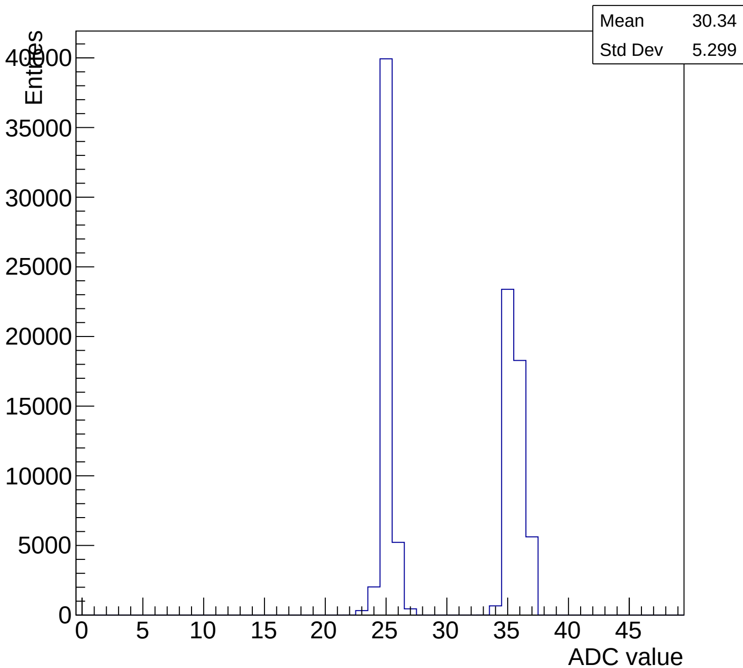
Pedestals ch 2 chip 65 run 20336 morecapacitors
