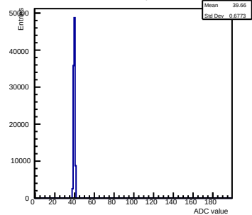
Pedestals ch 11 chip 65 incm=0.8
