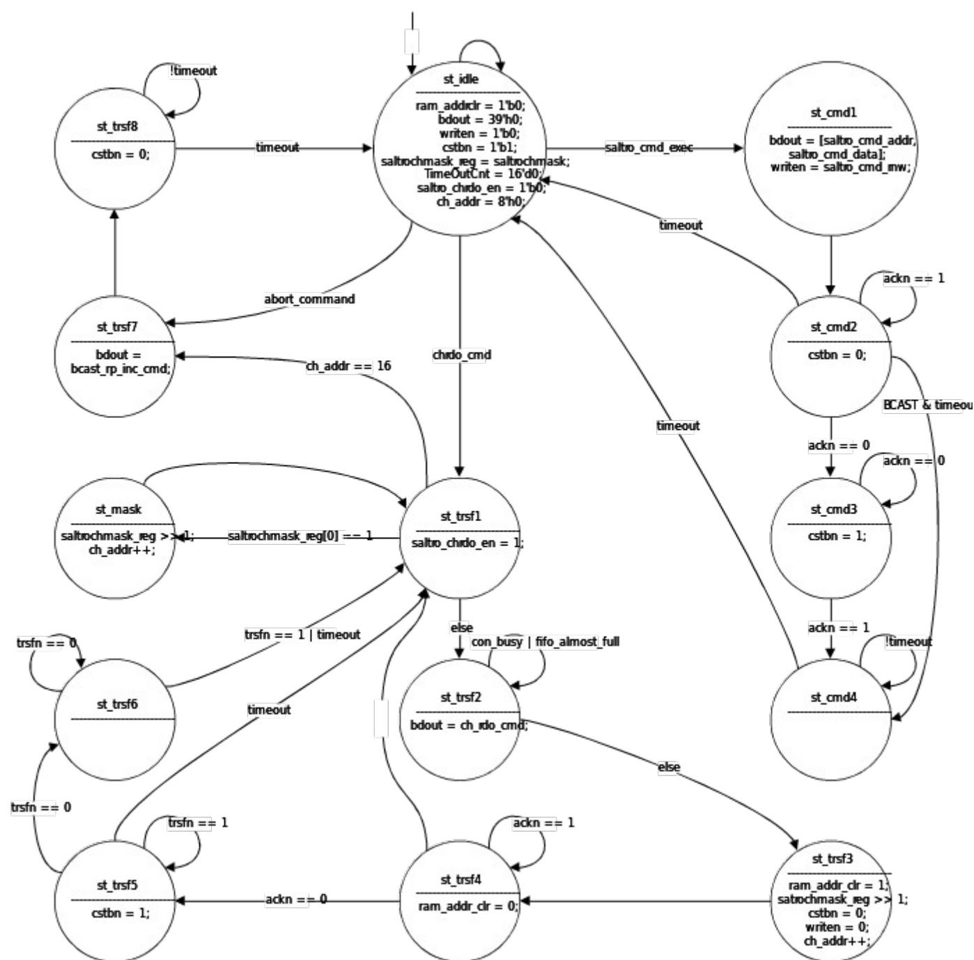
Figure 32: Saltro Controller CC FSM block diagram.
