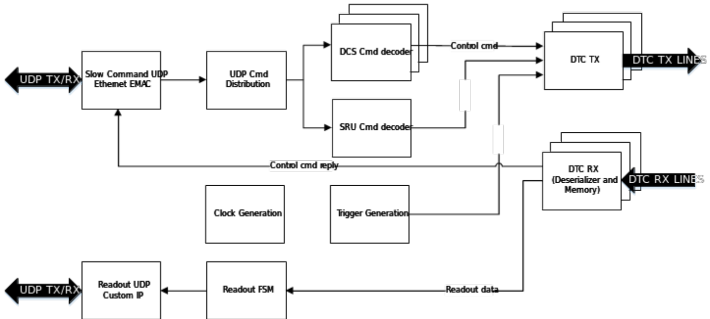
Figure 2: SRU architecture.
