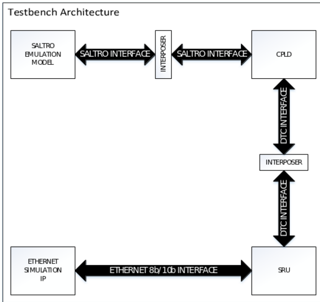
Figure 1: Testbench Architecture.
