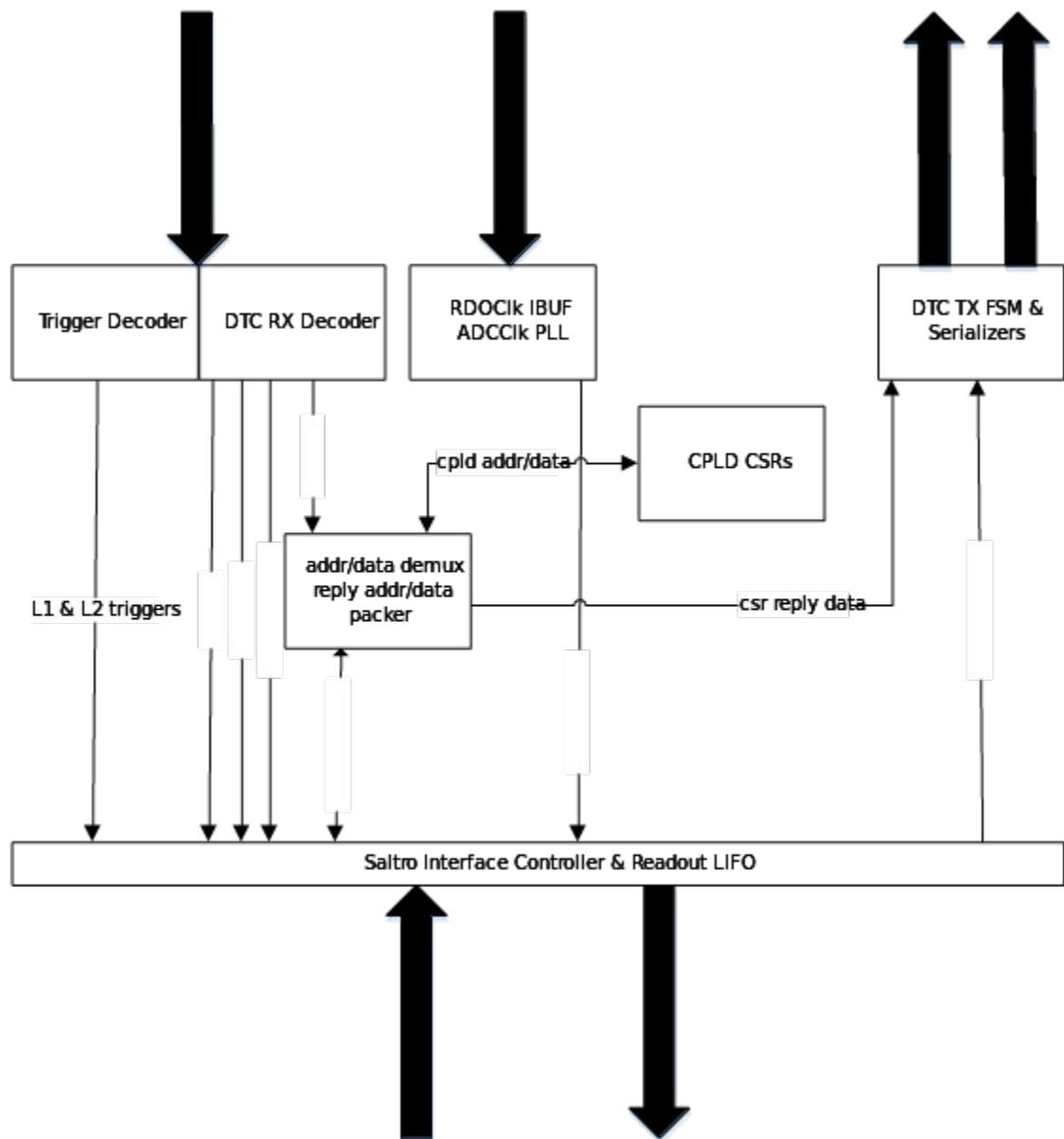
Figure 21: CPLD Architecture.
