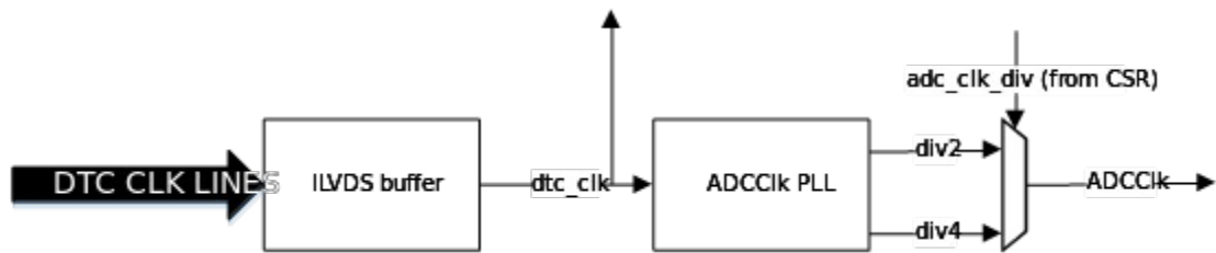
Figure 23: ADC clock PLL and DTC clock buffer.
