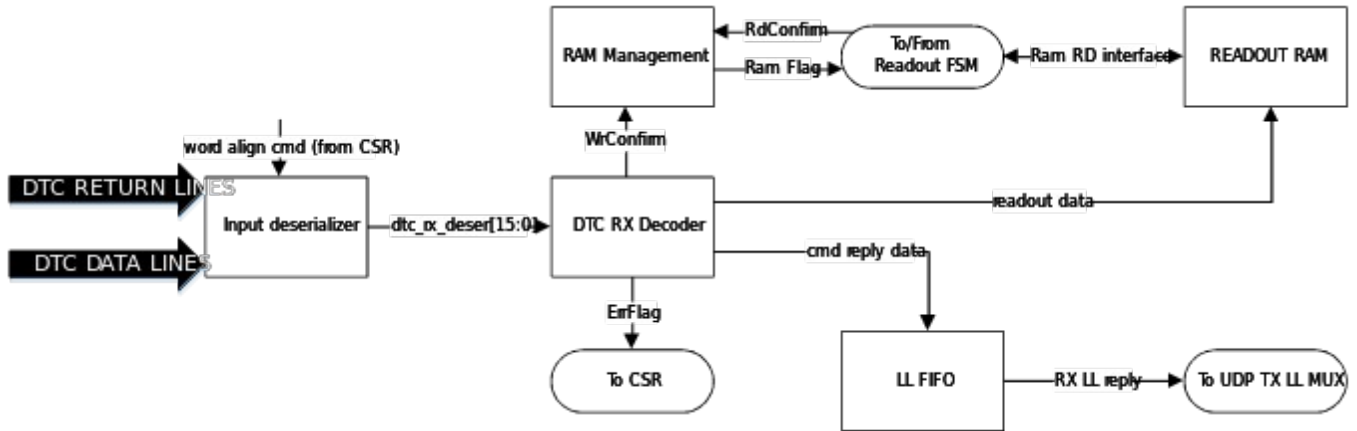
Figure 16: DTC RX block diagram.
