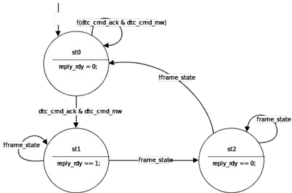
Figure 29: DTC Reply_Rdy FSM state diagram.
