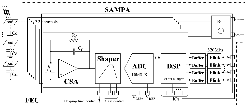
Figure 1: Block diagram for the SAMPA chip.
