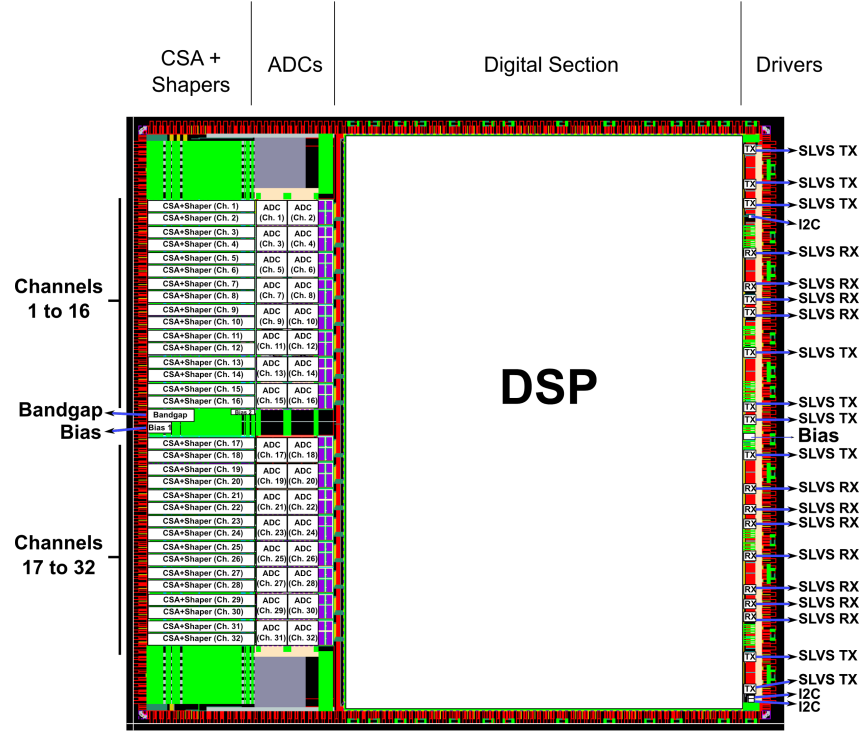
Figure 11: Full-chip with highlighted blocks
