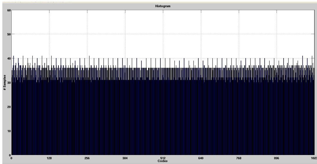
Figure 6. ADC full extracted simulation histogram, considering parasitic routing and dumping resistors.
