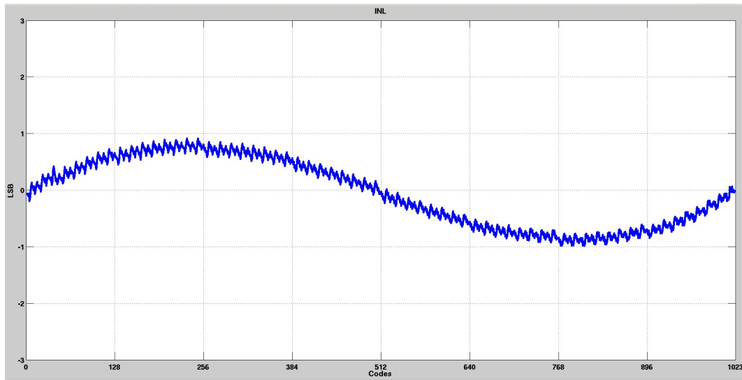
Figure 8. ADC full extracted simulation INL, considering parasitic routing and dumping resistors. INL < 1 \text{ LSB} .
