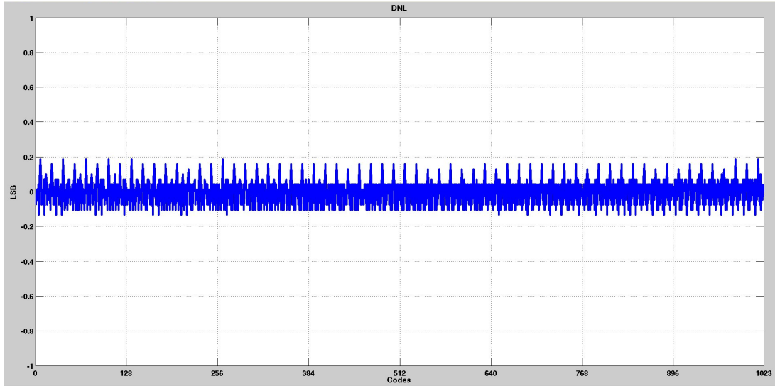
Figure 7. ADC full extracted simulation DNL, considering parasitic routing and dumping resistors. DNL < 0.2 \text{ LSB} .
