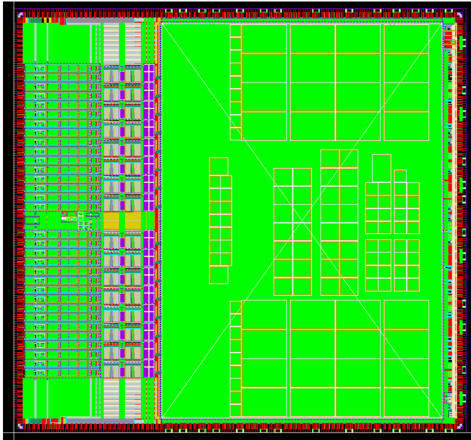
Figure 10: SAMPA V4 full layout.
