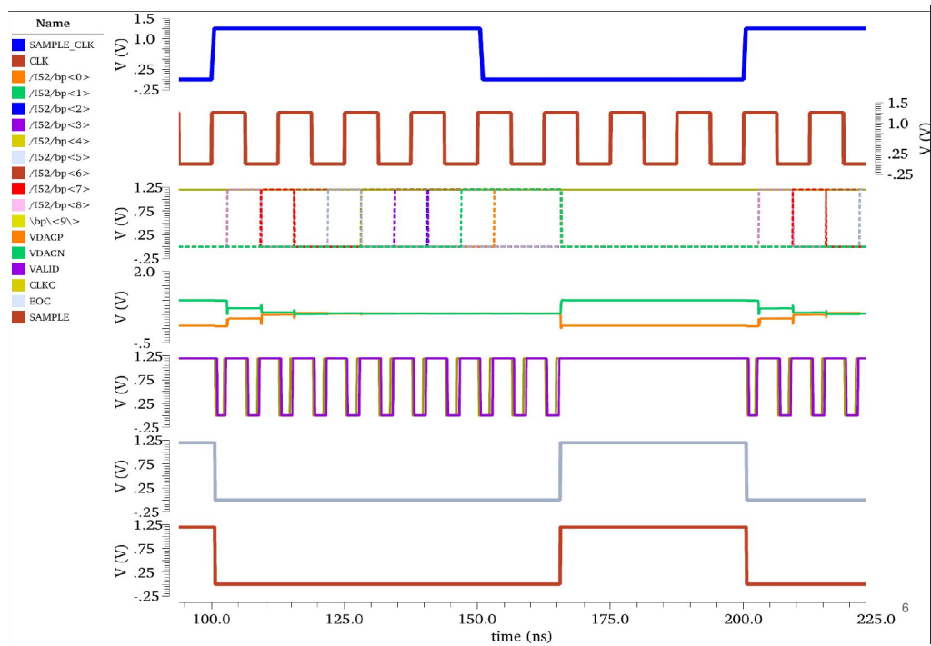
Figure 4. ADC Time diagram.
