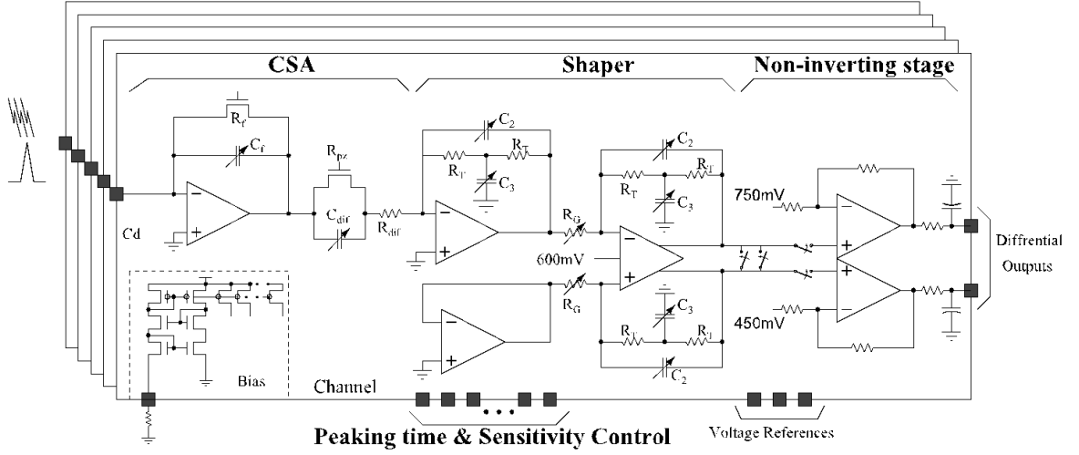
Figure 2: Block diagram of the analog front-end.
