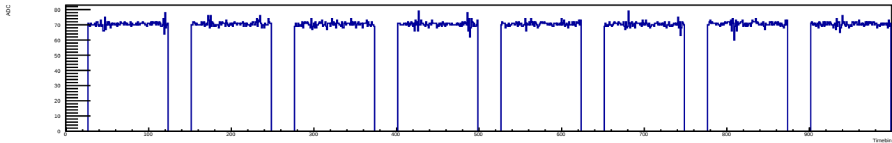
Sweep 0 for chip 1601 chan 30
