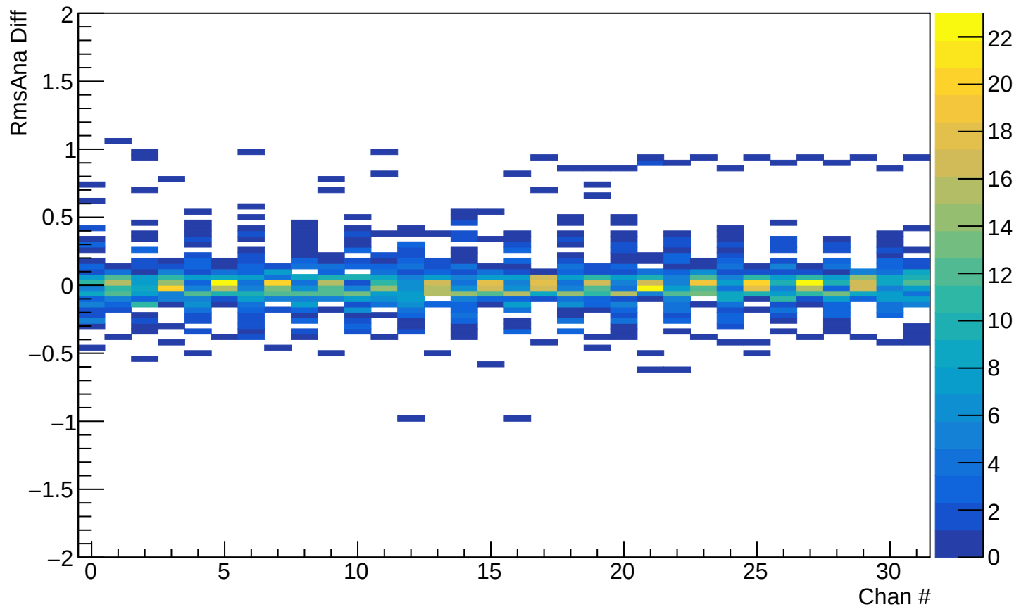
DiffRmsAna vs Chan : Sta 0
