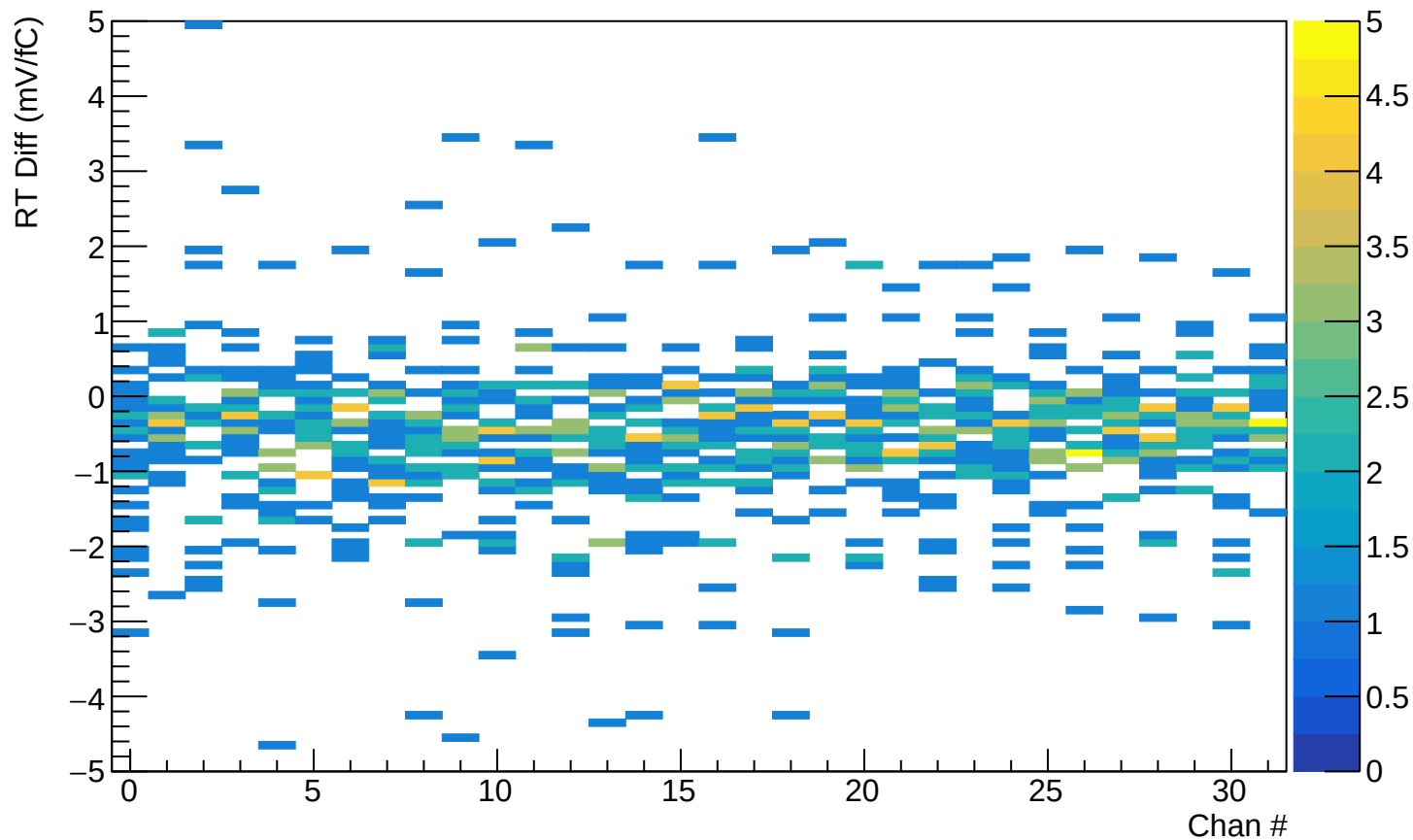
DiffRT vs Chan : Sta 1
