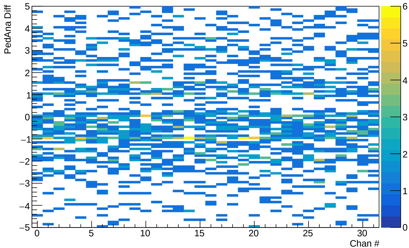
DiffPedAna vs Chan : Sta 1
