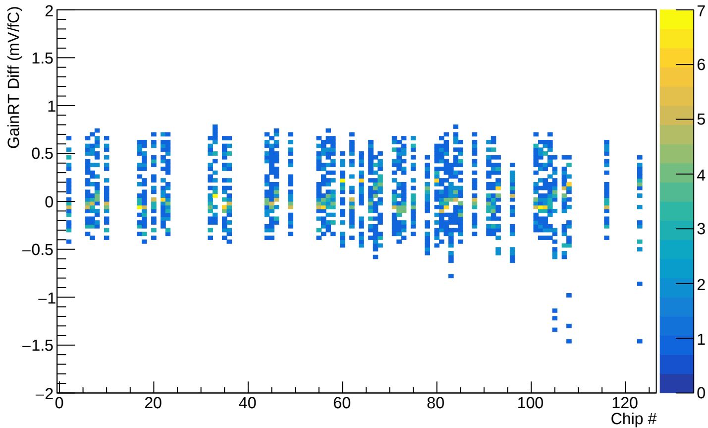
DiffGainRT vs Chip : Sta 0
