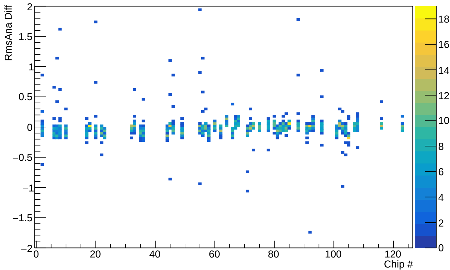
DiffRmsAna vs Chip : Sta 0
